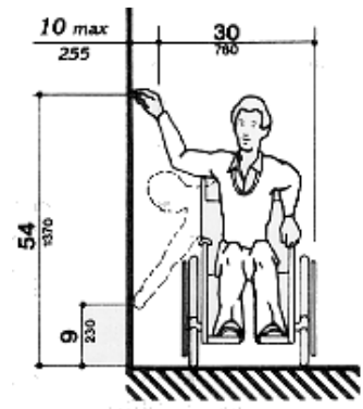
Figure 6b. Parallel approach - high/low side reach.
