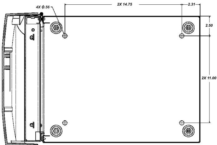
Fig. 11. Mounting hole drill template example (Not to scale).
