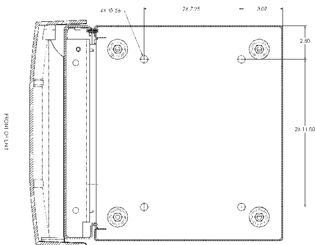
Fig. 10. Mounting hole drill template example (Not to scale).
