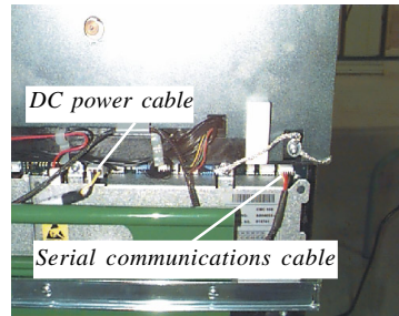
Figure 3. Disconnect the DC power and serial communication connectors from the dispensing mechanism.
