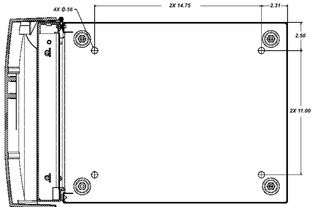
9700/9750/9720/9770 ANCHOR DRILL TEMPLATE
