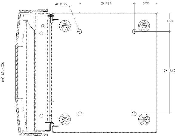
9700/9750/9720/9770 ANCHOR DRILL TEMPLATE
