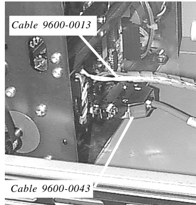
Figure 3. Connections for DC power and communications.
