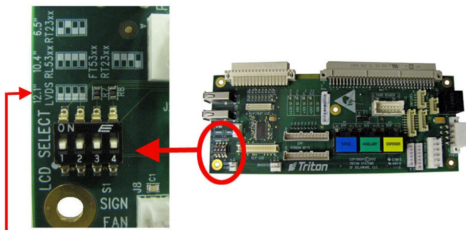
(photo above shows the switches set for the 12.1" display, all switches in the OFF position)
